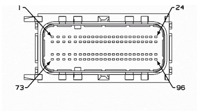
Mating Side:
