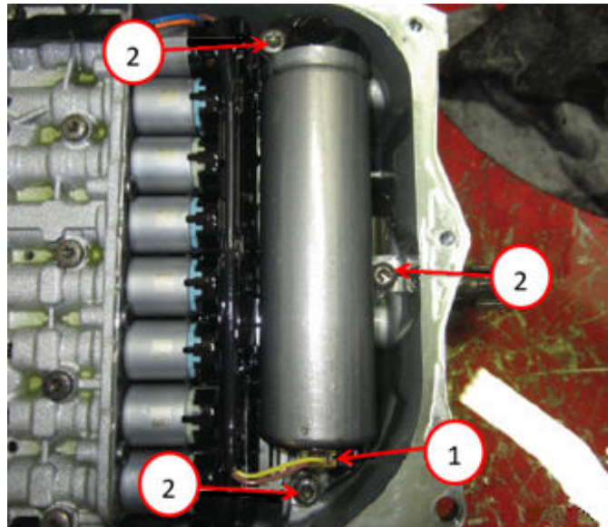
Fig. 8 Hydraulic Impulse Oil Storage
