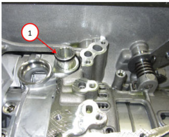
Fig. 13 Fluid Port
